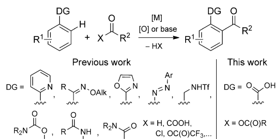
Scheme 1. Previous work on C–H bond acylation. DG = directing group, Tf = trifluoromethanesulfonyl.
